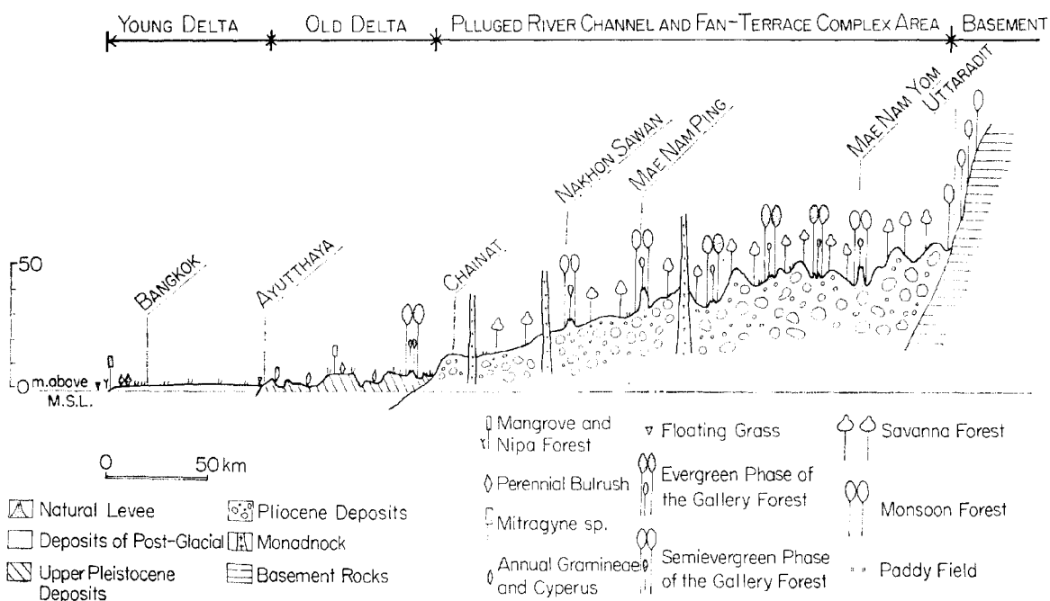
Fig. 3 N-S Cross-Section through Bangkok, Ayutthaya, Chainat and Uttaradit, showing the Relationship between Vegetations and Physiography
