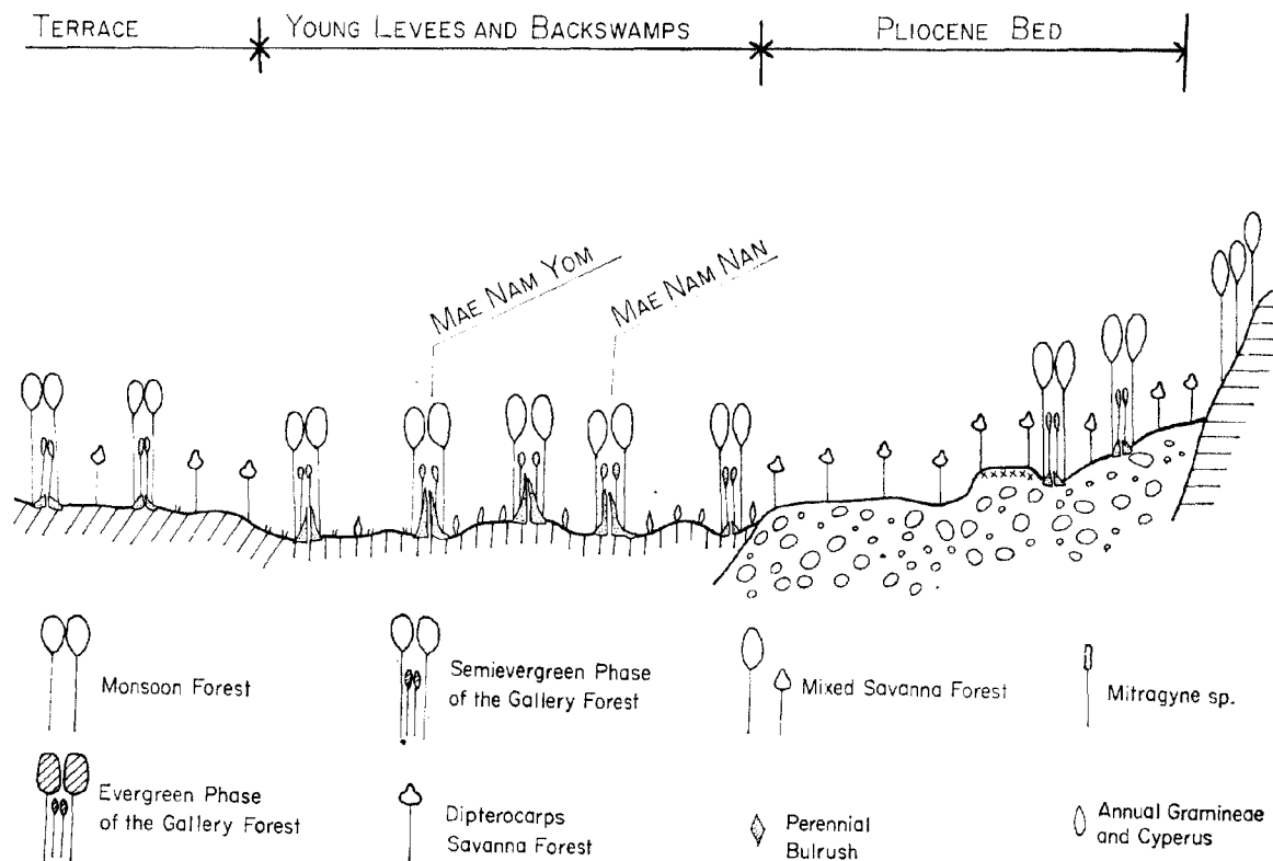
showing the Relationship between Vegetations and Physiography
