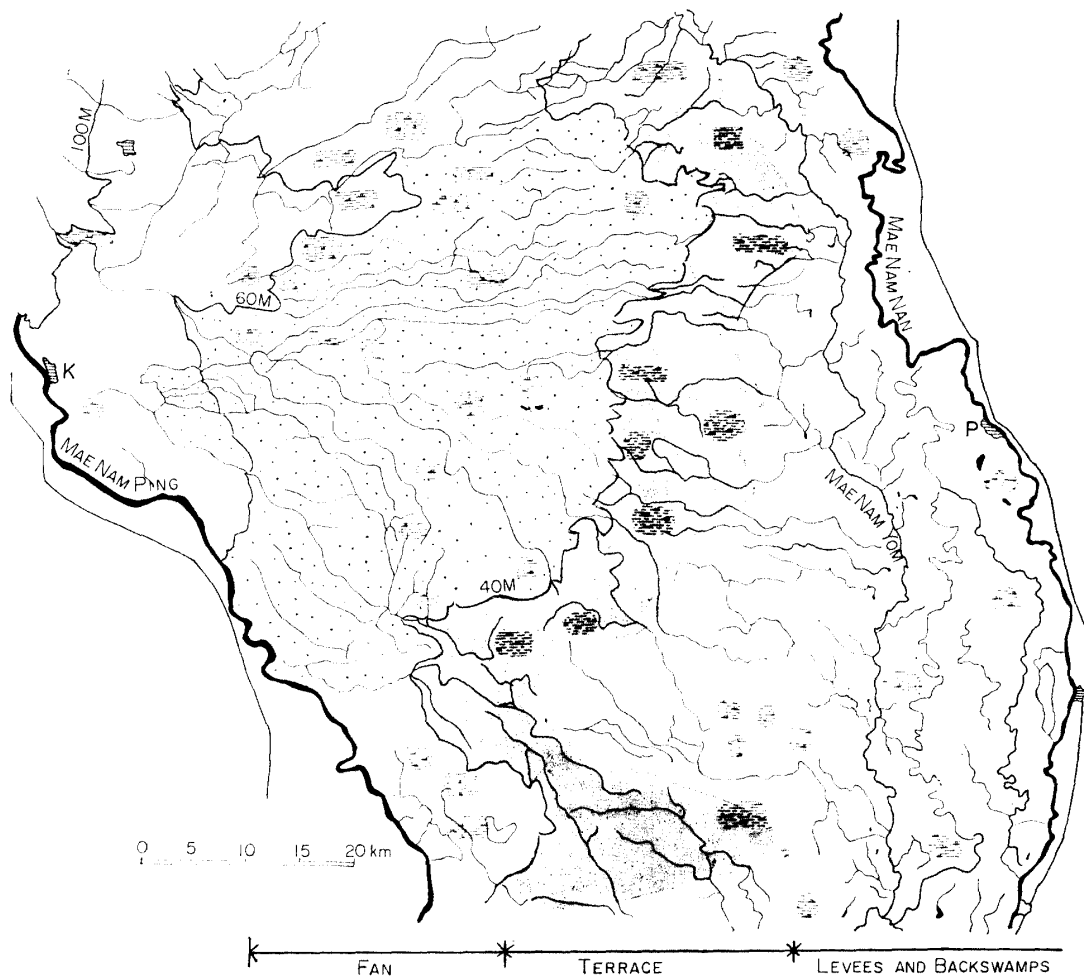
Fig. 1 A Physiographical Map, showing the Fan-Terrace Complex and Plugged River Channel Areas
