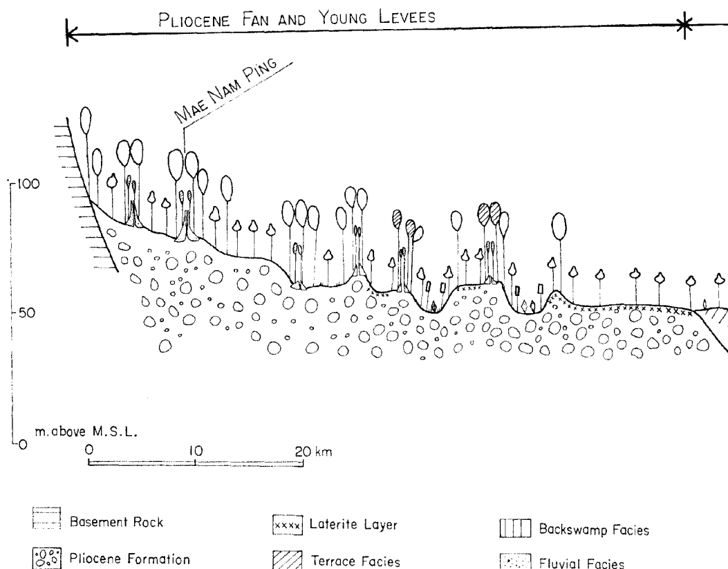
Fig. 2 E-W Cross-Section along the Line of Long. 80°20'E,
